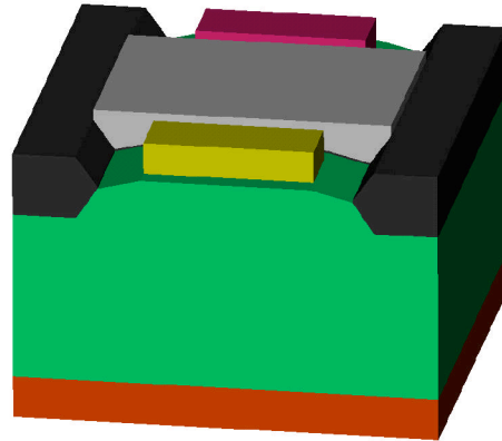
Figure 1. Seven region geometry solid geometry model. The 'air' region has been removed for viewing. All bounding surfaces are planes.
