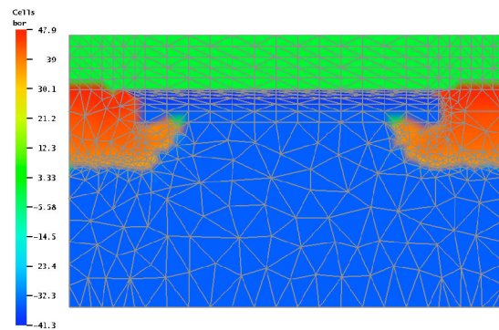
Figure 7. Results of refinement, smoothing and reconnection.
